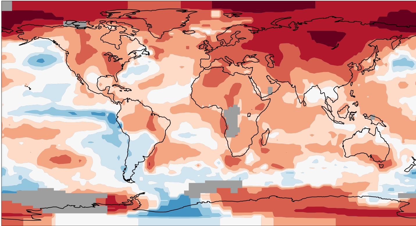
Surface Temperature Anomaly ( ^{\circ}\text{C} )
