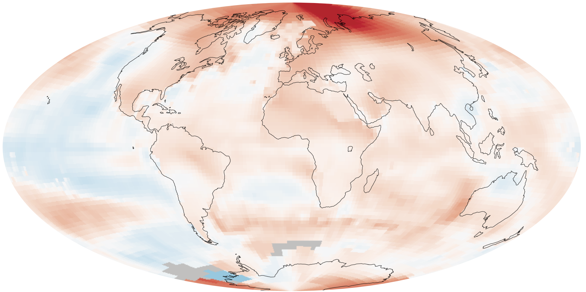
2011 Global Temperature Difference (°C) -4 -2 0 +2 +4
