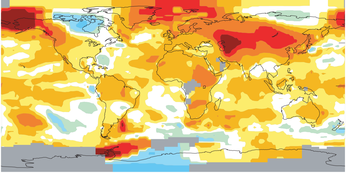
2004 Annual Mean Surface Temperature Anomalies (°C)
