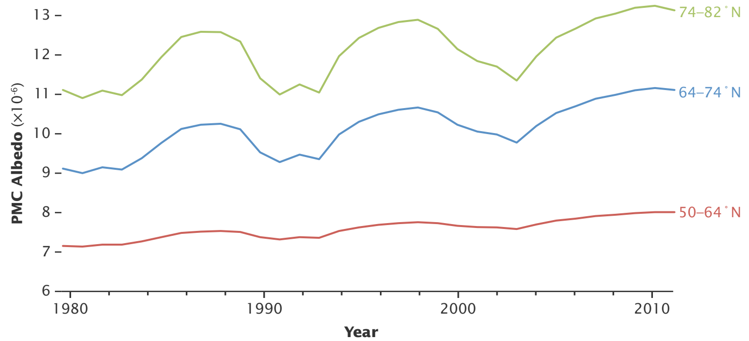
Increase of Polar Mesospheric Clouds, 1979–2010
