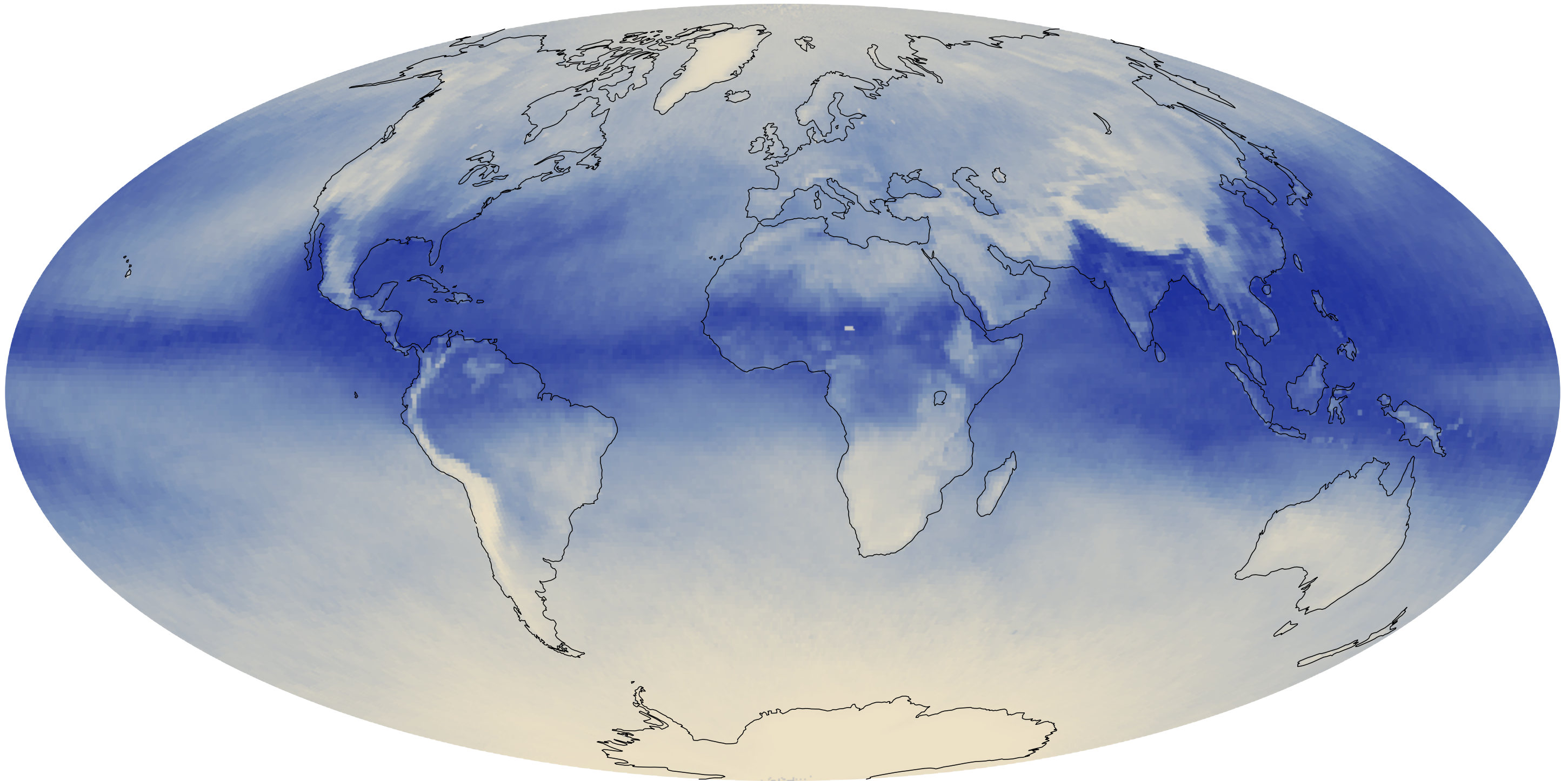
Total Precipitable Water (mm)
