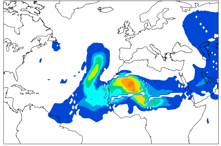
Modelled Aerosol (GOCART Aerosol Index)
