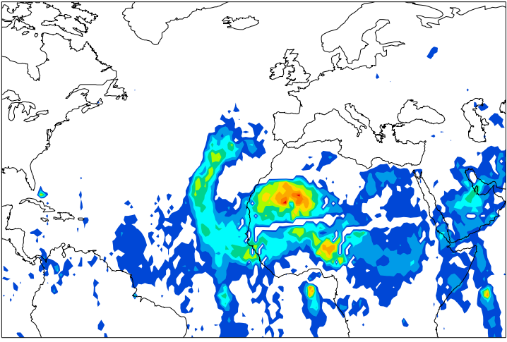
Measured Aerosol (TOMS Absorbing Aerosol Index)
